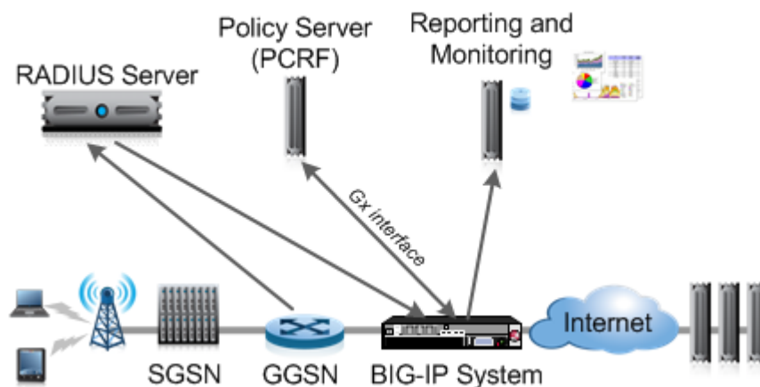
Figure 1: Diagram of policy enforcement overview
